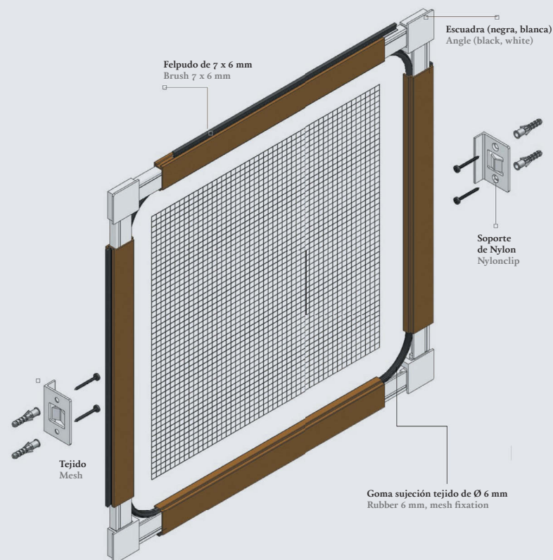
Explosionado mosquitera Fija Belle Mare Exploded view Fixed insect screen Belle Mare
