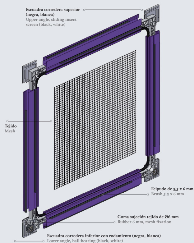
Explosionado mosquitera Corredera Belle Mare Exploded view Sliding insect screen Belle Mare
