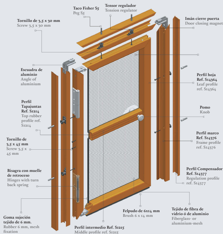
Explosionado mosquitera Abatible Copacabana Exploded view Hinged Door insect screen Copacabana
